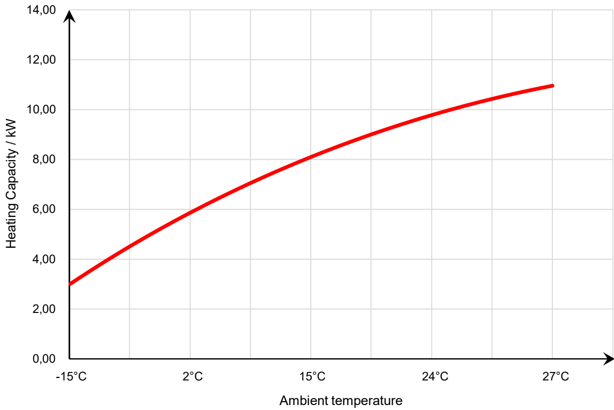
34-180501 Heating Capacity Curve
