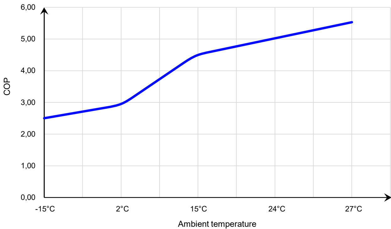
34-180502 COP Curve
