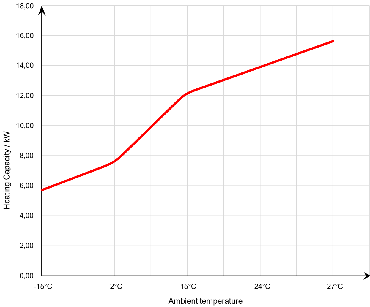
34-180502 Heating Capacity Curve
