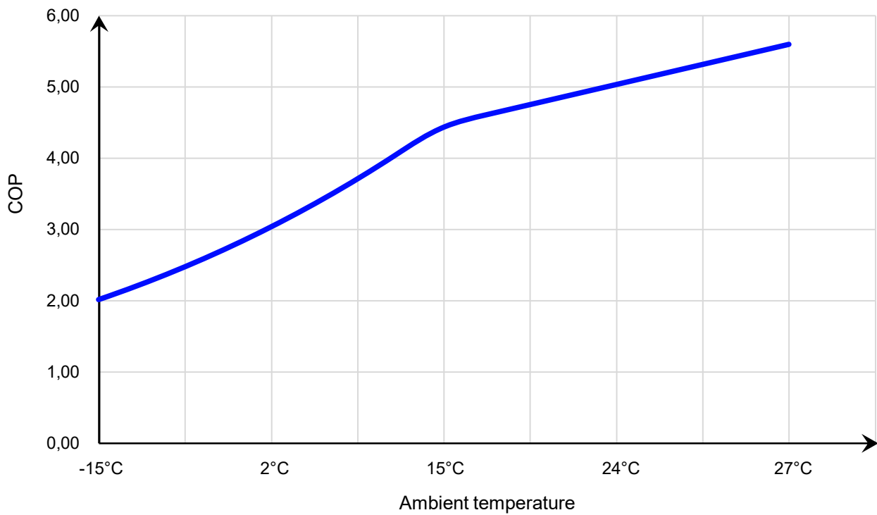
34-180501 COP Curve
