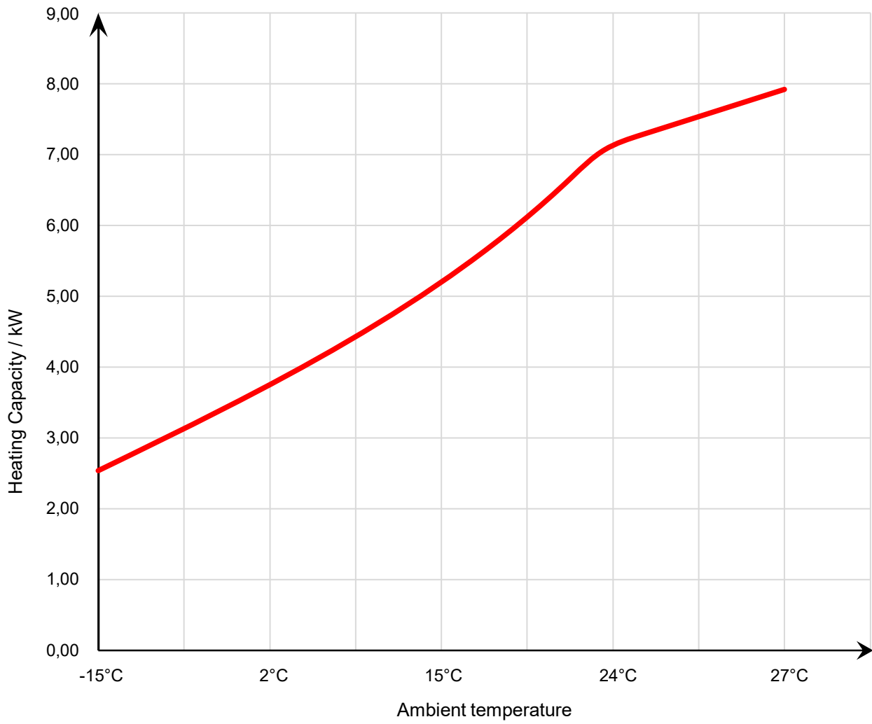
34-180610 Heating Capacity Curve
