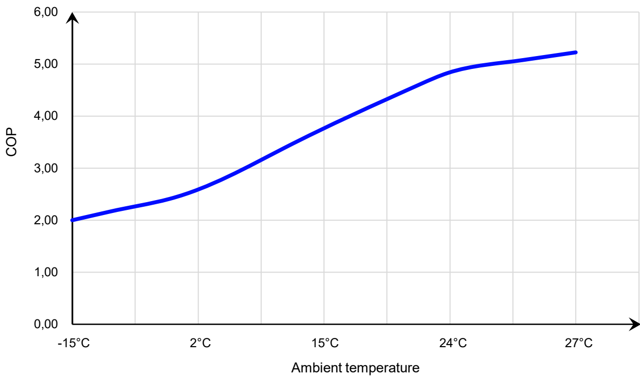
34-180614 COP Curve
