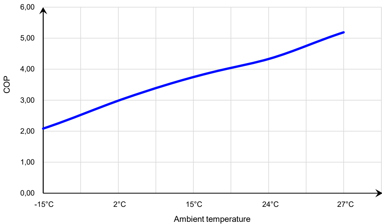
34-180610 COP Curve
