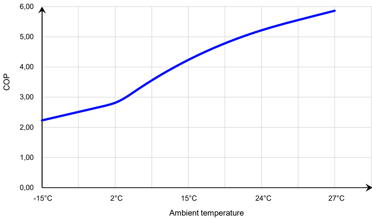
34-180612 COP Curve
