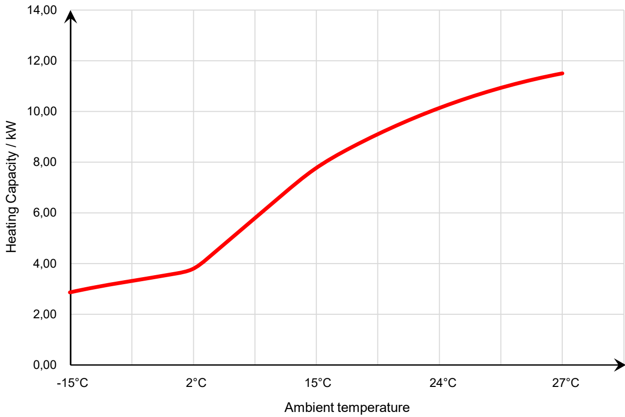
34-180612 Heating Capacity Curve
