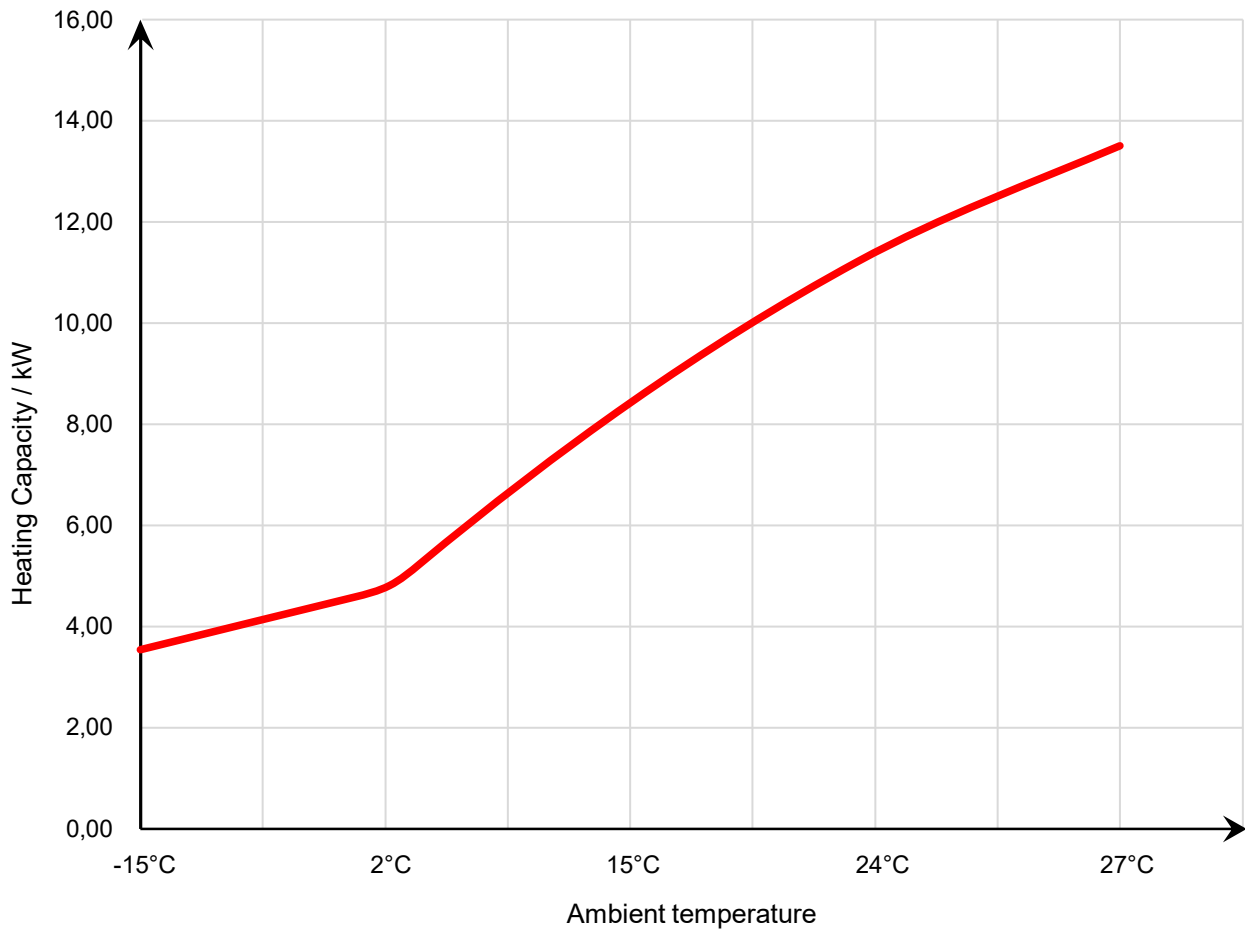
34-180614 Heating Capacity Curve
