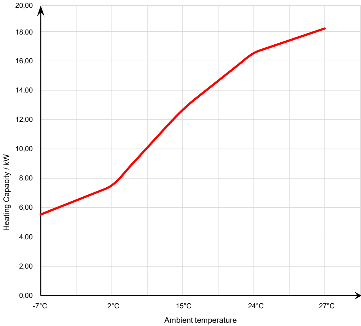
34-180626 Heating Capacity Curve
