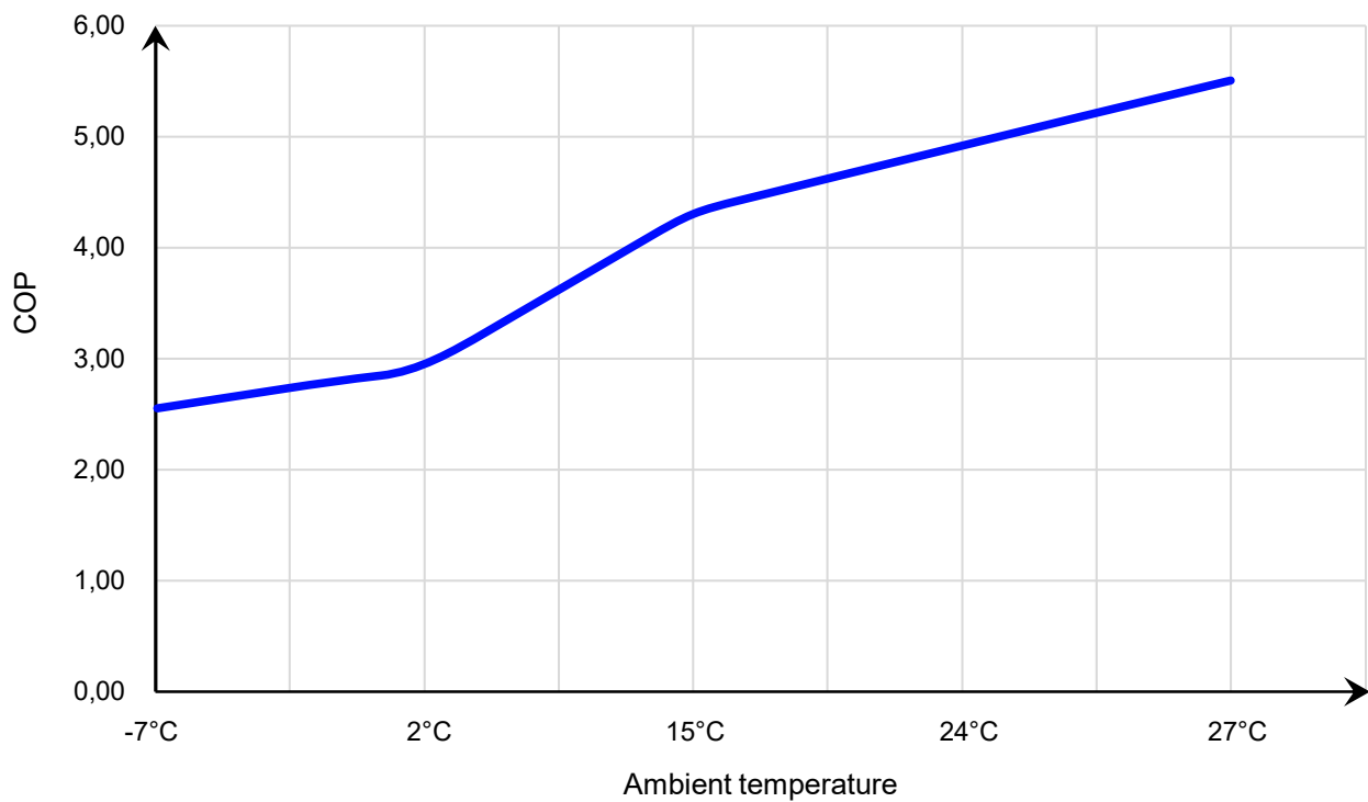
34-180624 COP Curve
