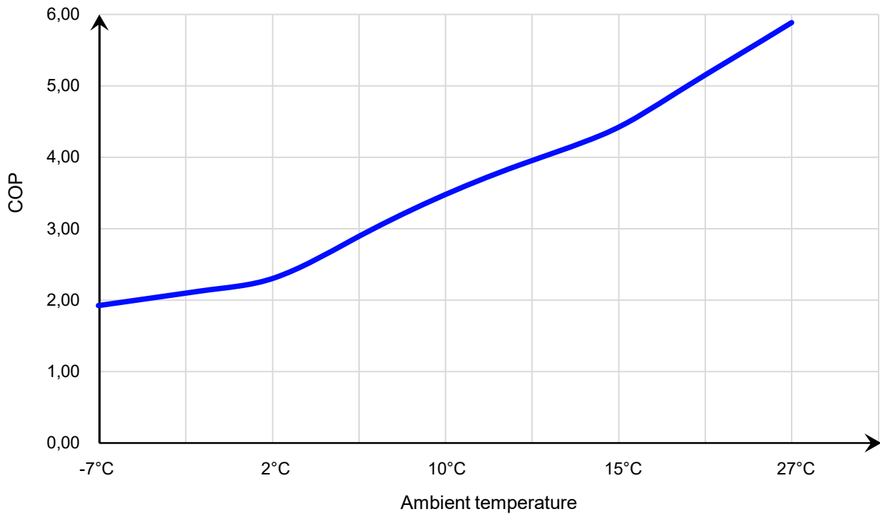
34-180620 COP Curve
