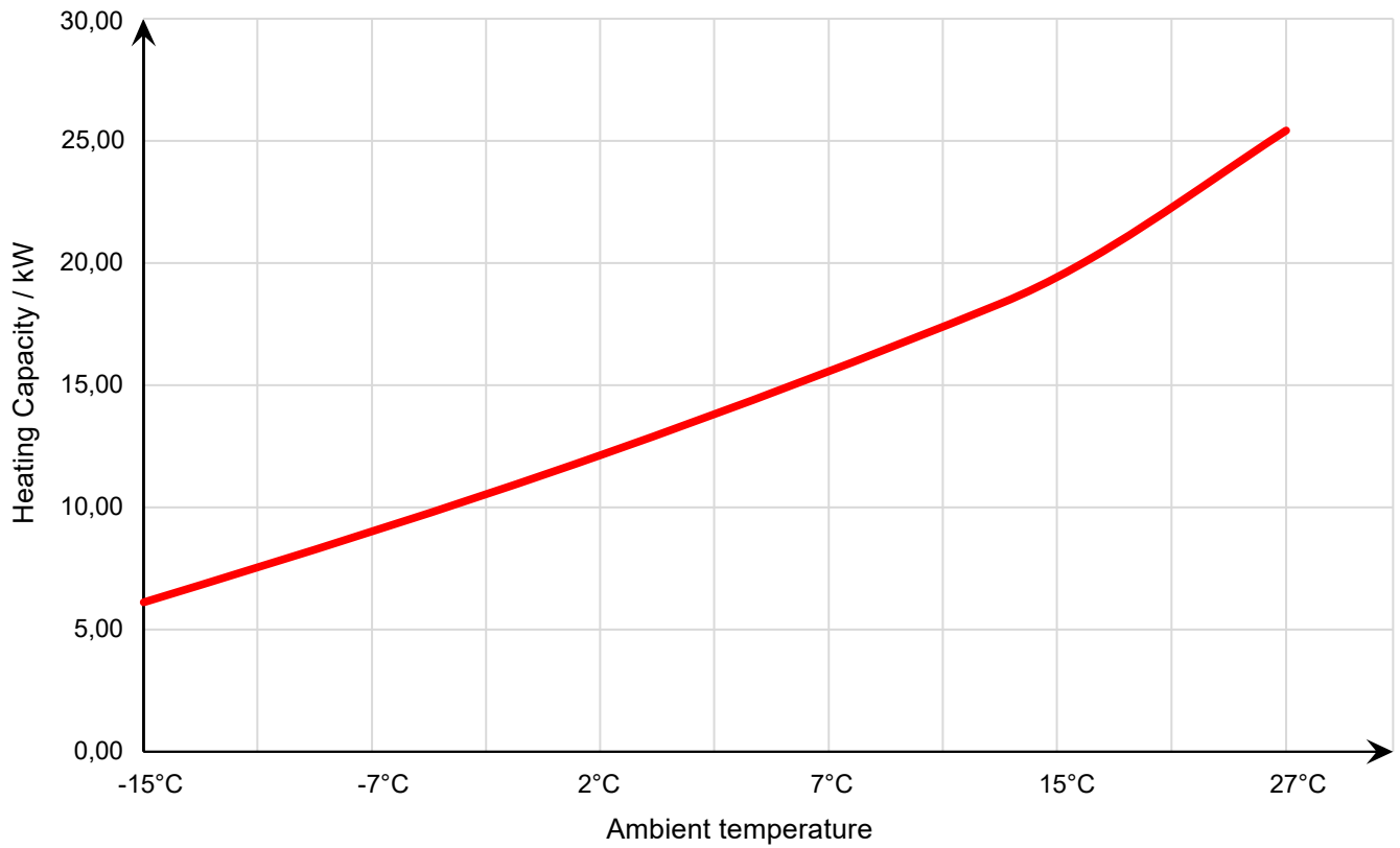
34-180640 Heating Capacity Curve
