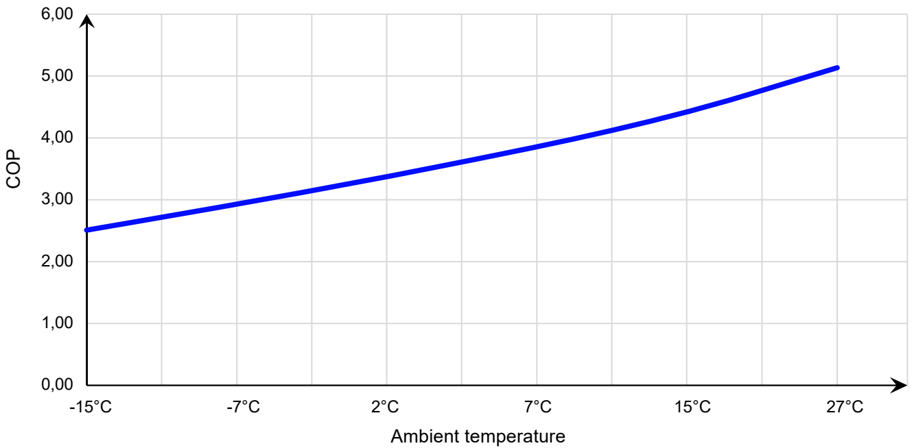
34-180642 COP Curve
