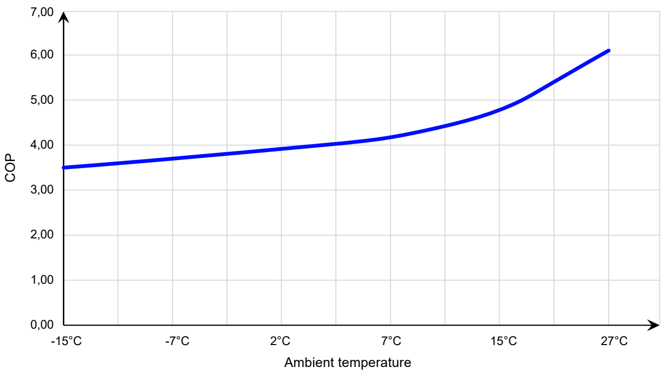
34-180628 COP Curve
