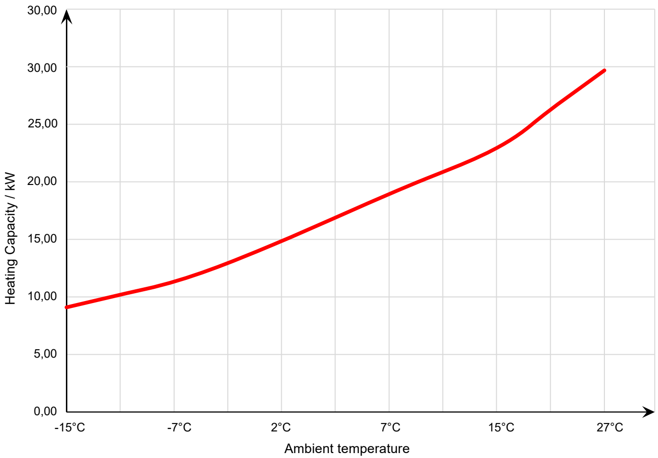
34-180642 Heating Capacity Curve
