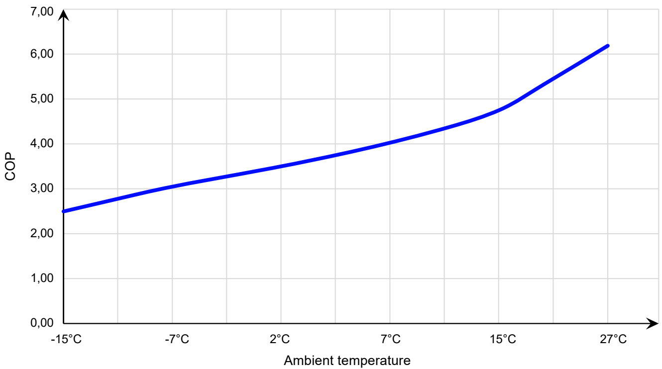
34-180640 COP Curve
