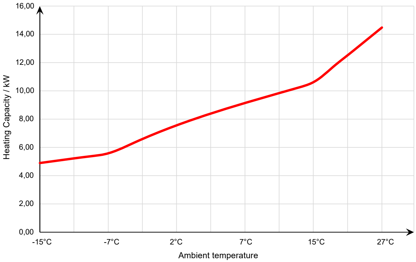
34-180628 Heating Capacity Curve
