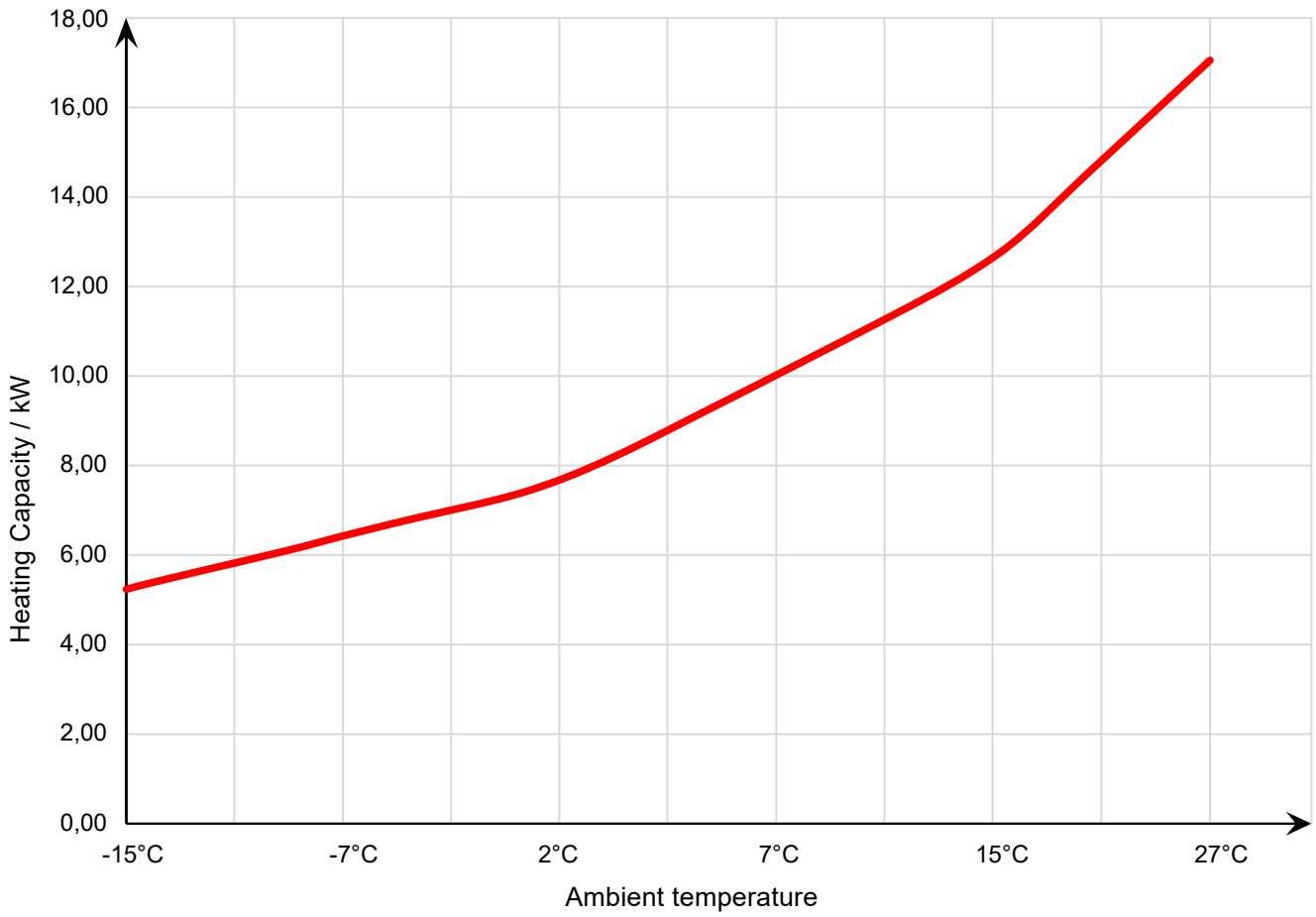
34-180630 Heating Capacity Curve
