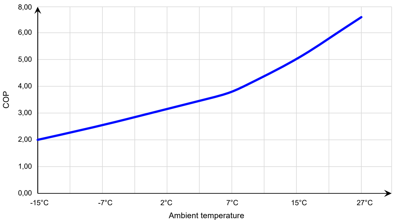
34-180630 COP Curve
