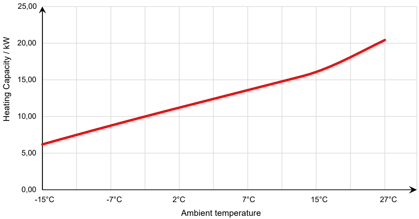
34-180632 Heating Capacity Curve
