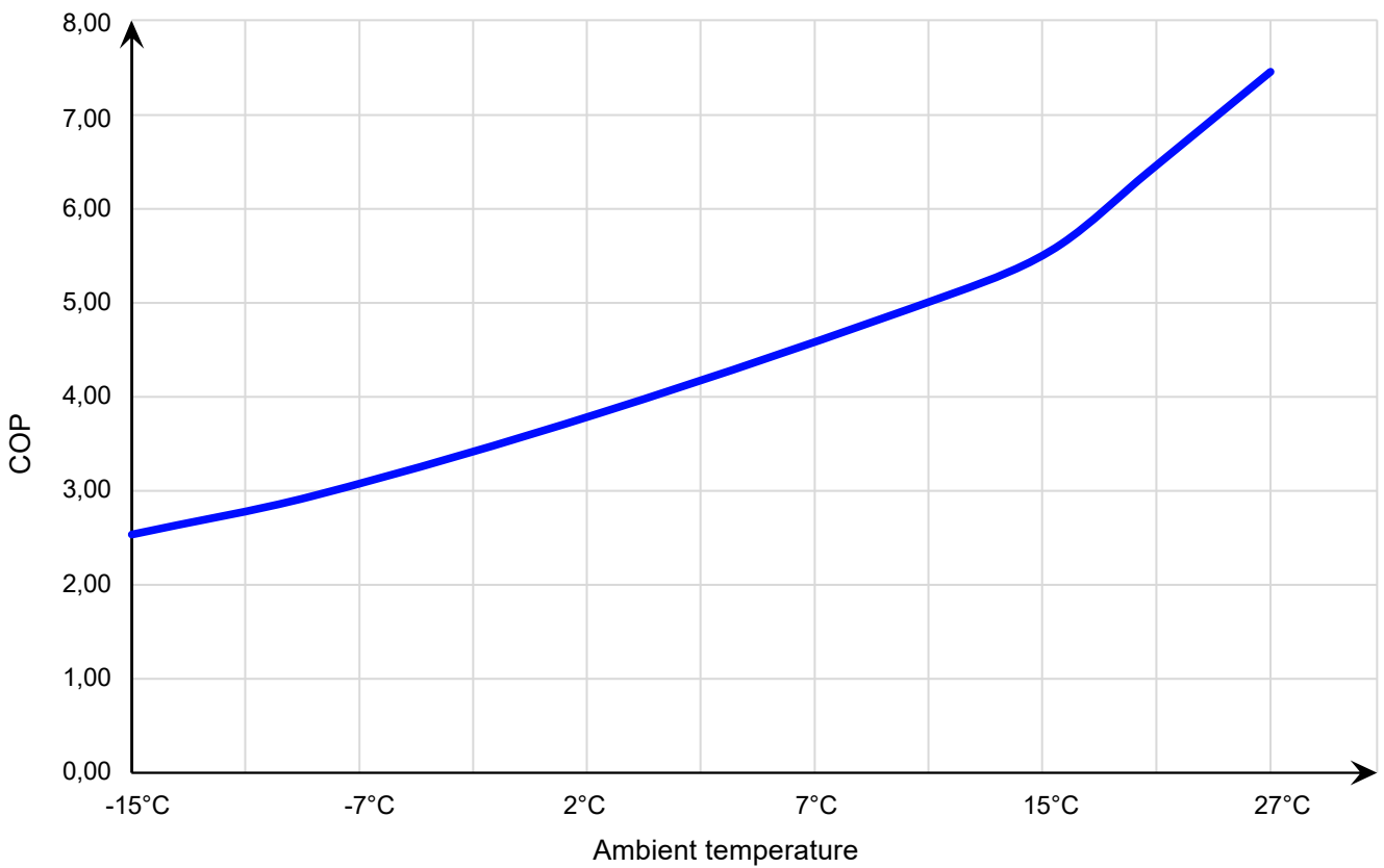
34-180632 COP Curve
