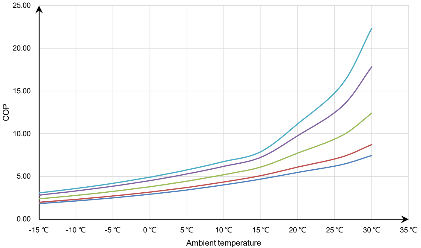
34-180656 COP Curve
