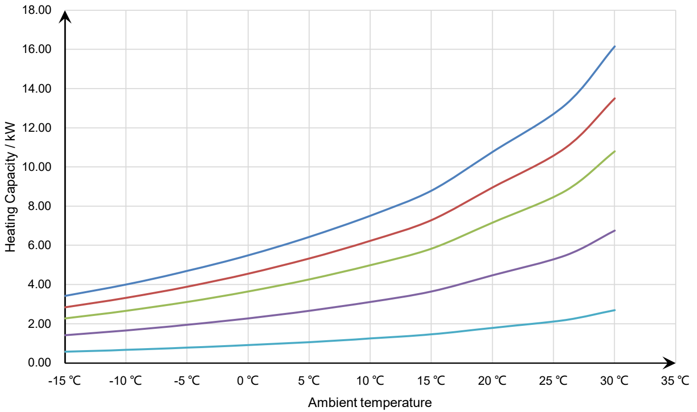
34-180652 Heating Capacity Curve
