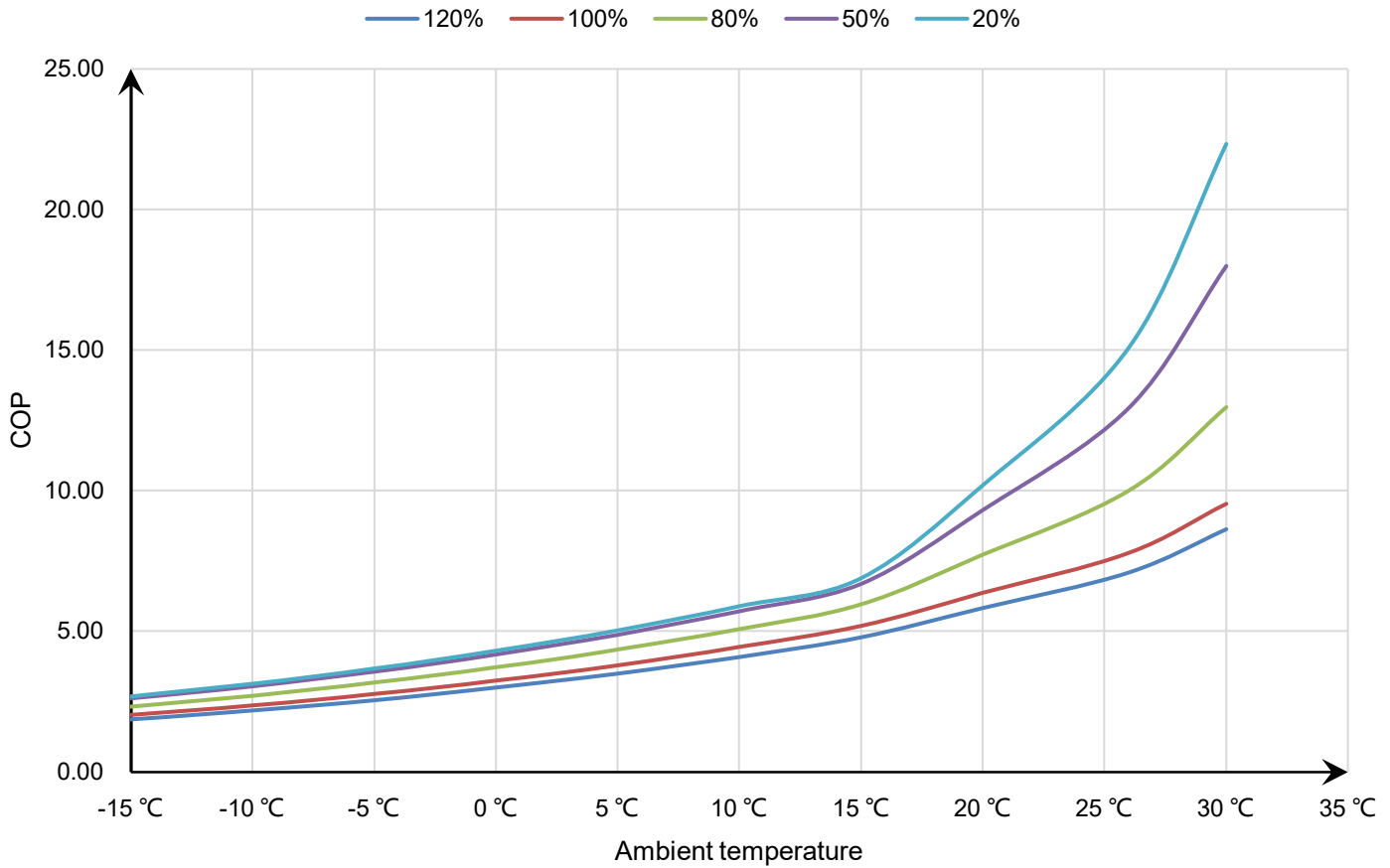
34-180650 COP Curve
