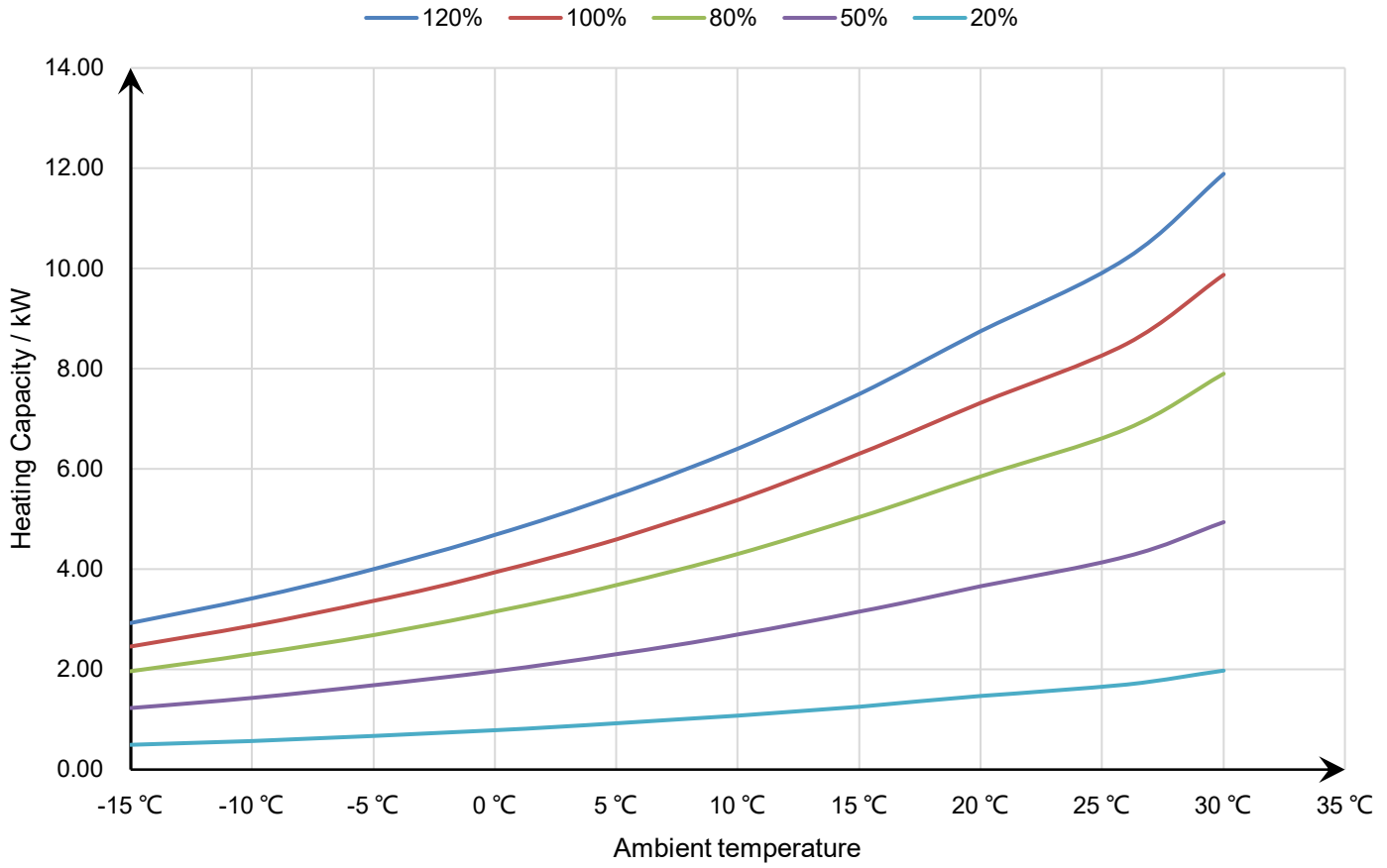
34-180650 Heating Capacity Curve
