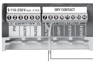
Setup and connection of a Variable Speed Pump, see section 13 - Variable Speed Pump
