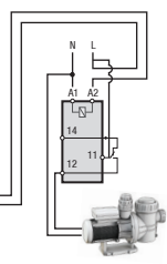
FILTER PUMP Filtration control ⑦ & ⑧
