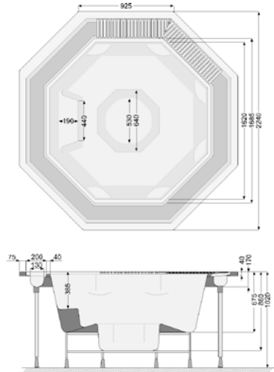
OCTAVIA PUBLIC VERSION WITH OVERFLOW
