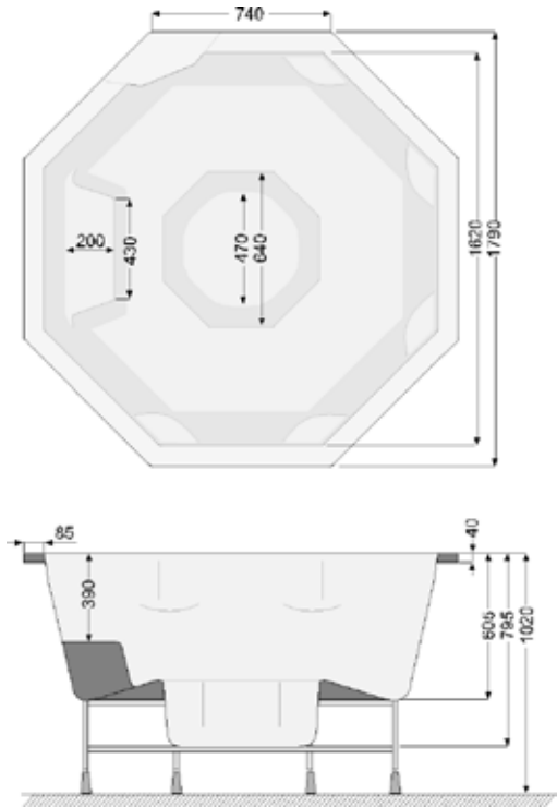
OCTAVIA PRIVATE VERSION WITH SKIMMER
