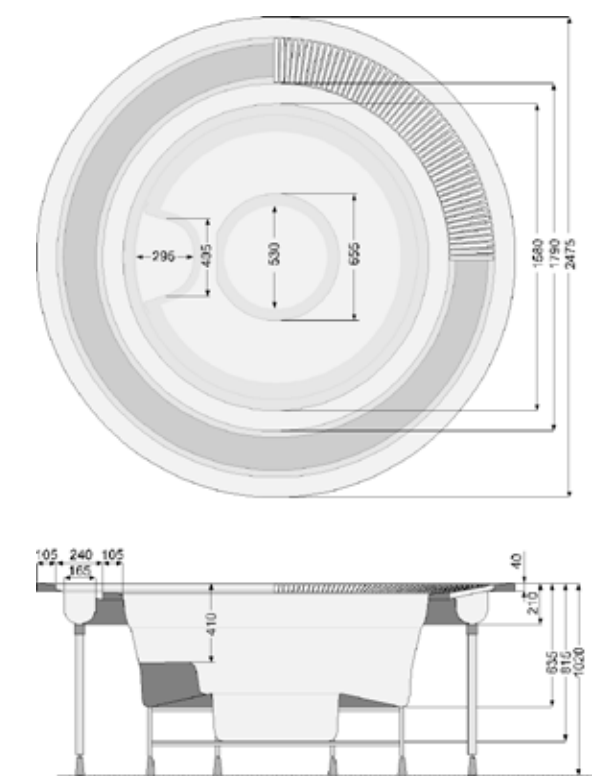
VICTORIA PUBLIC VERSION WITH OVERFLOW
