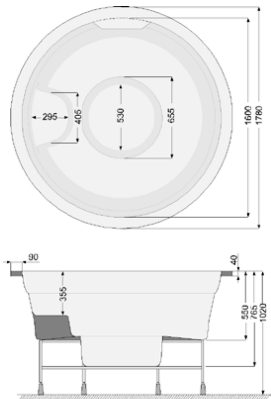
VICTORIA PRIVATE VERSION WITH SKIMMER
